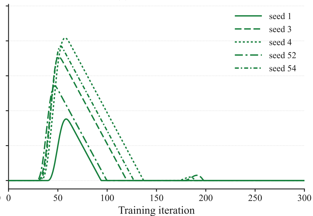
(b) cPPO, d = 15
