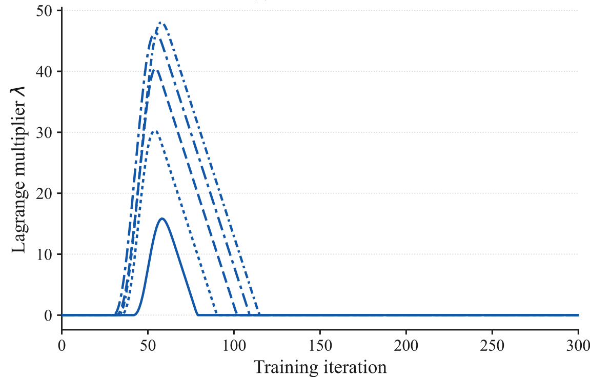
(a) cPPO, d = 25
