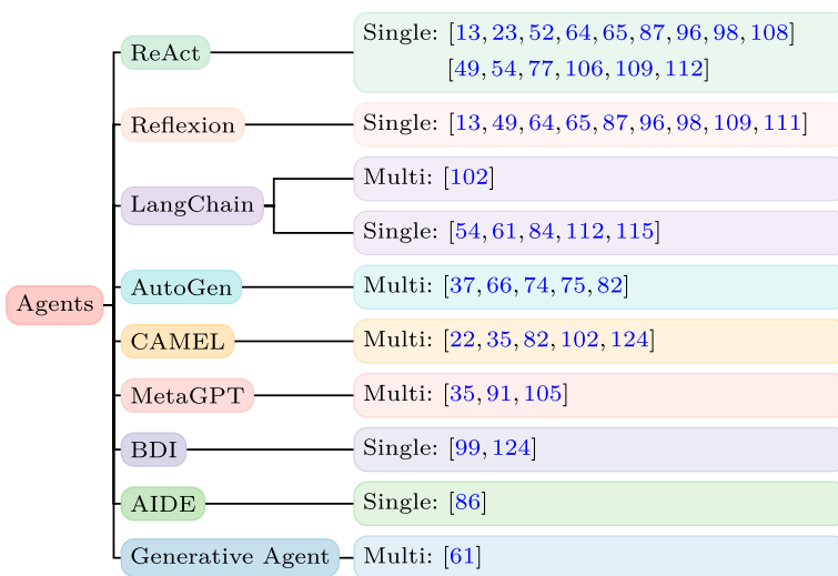
Fig. 6 Common LLM agent frameworks used in single- and multi-agent LLMs
