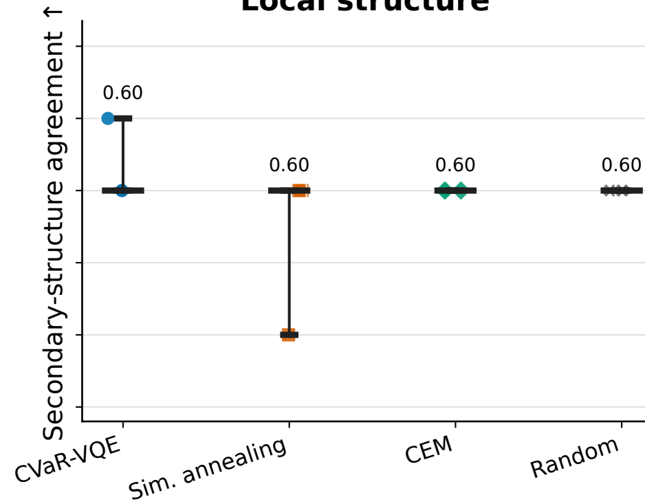
Local structure
