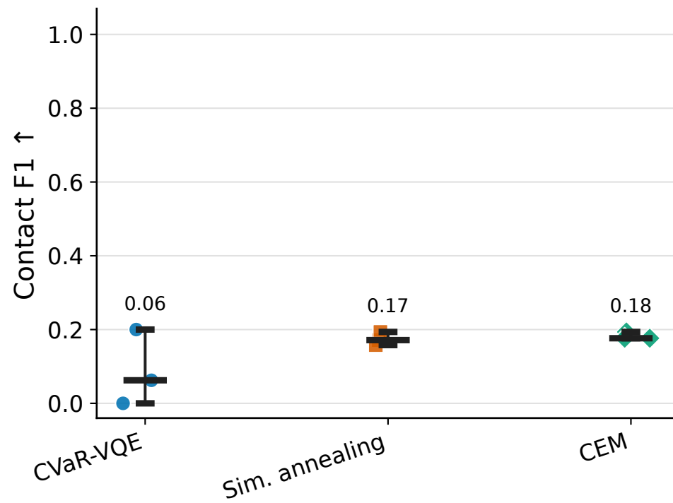
Native contacts
