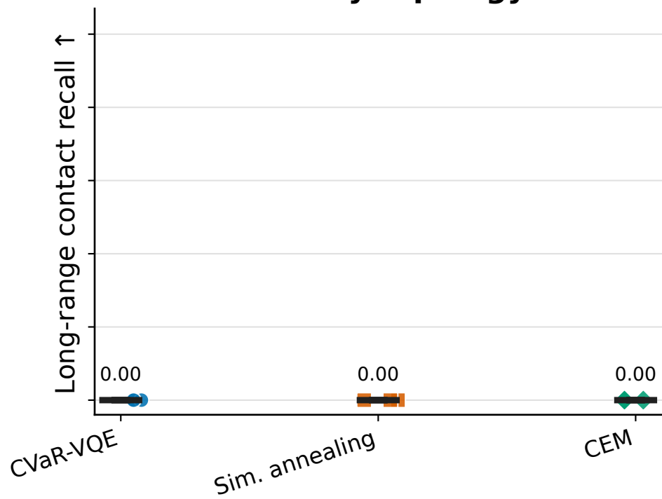
Tertiary topology
