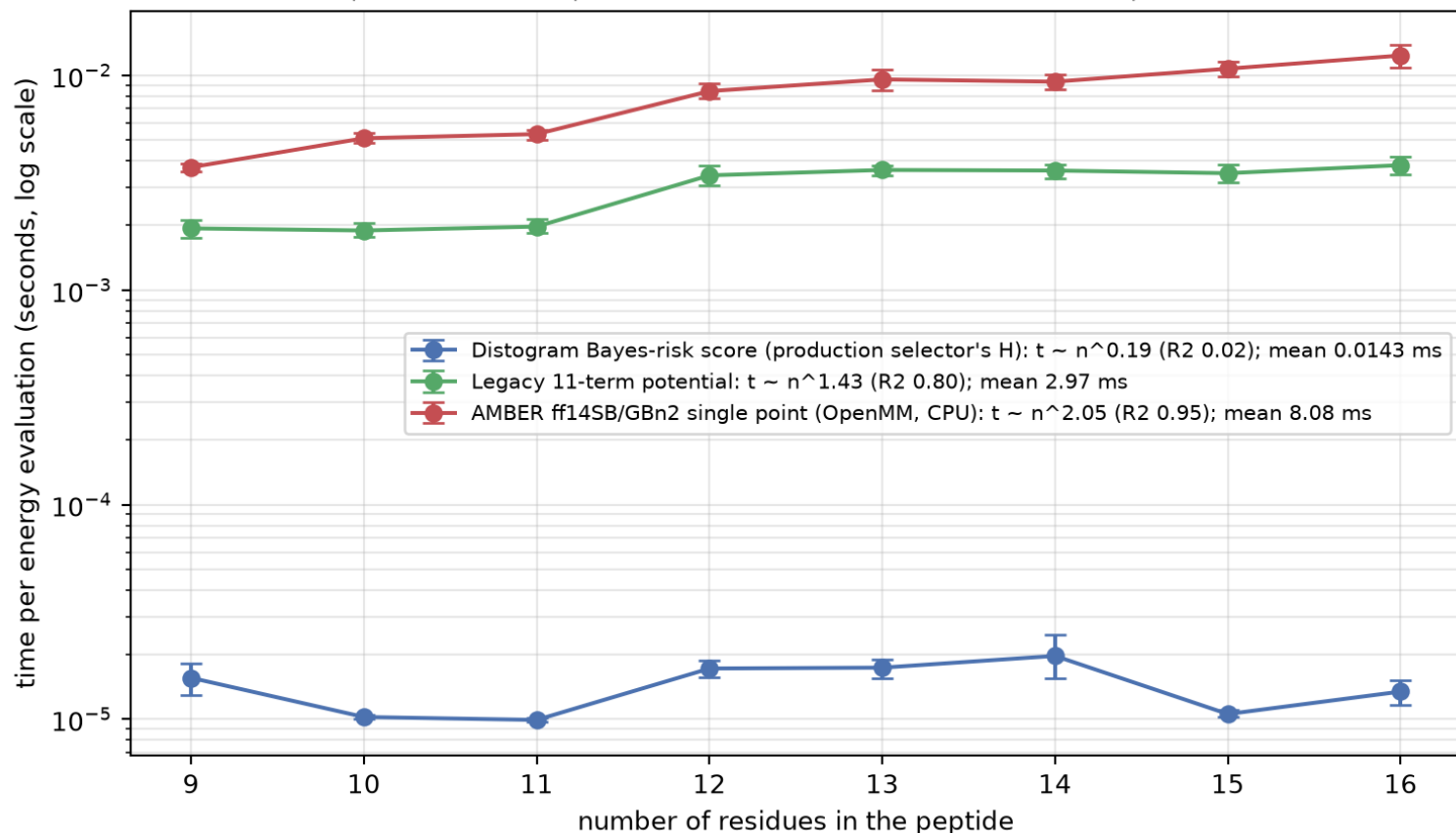
Time per single-structure energy evaluation versus peptide length 24 dev targets (3 per length) x 10 candidates x 5 repeats points = mean of per-candidate medians; error bars = bootstrap 95% CI
