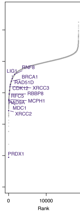
DNAPKi
