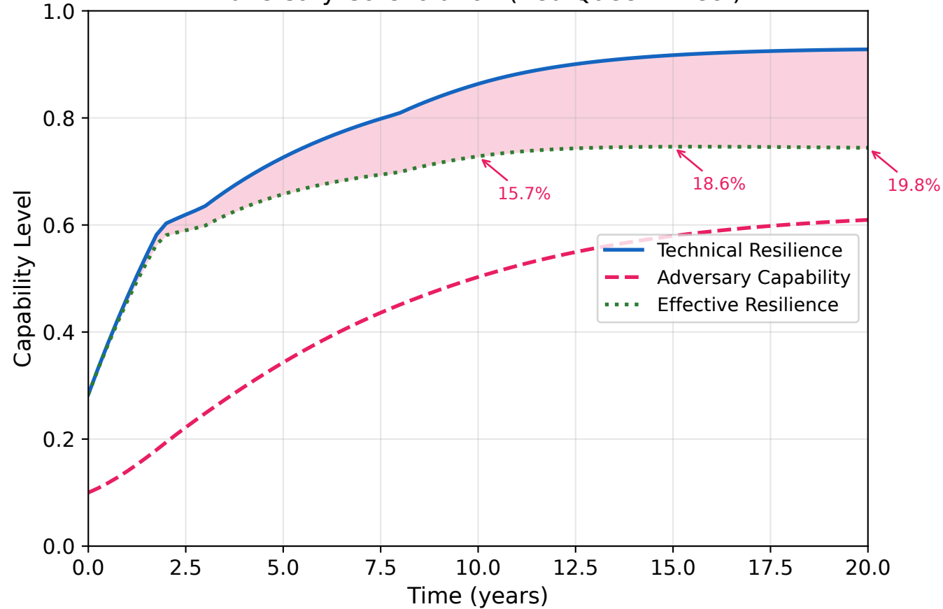
Adversary Co-evolution (Red Queen Effect)
