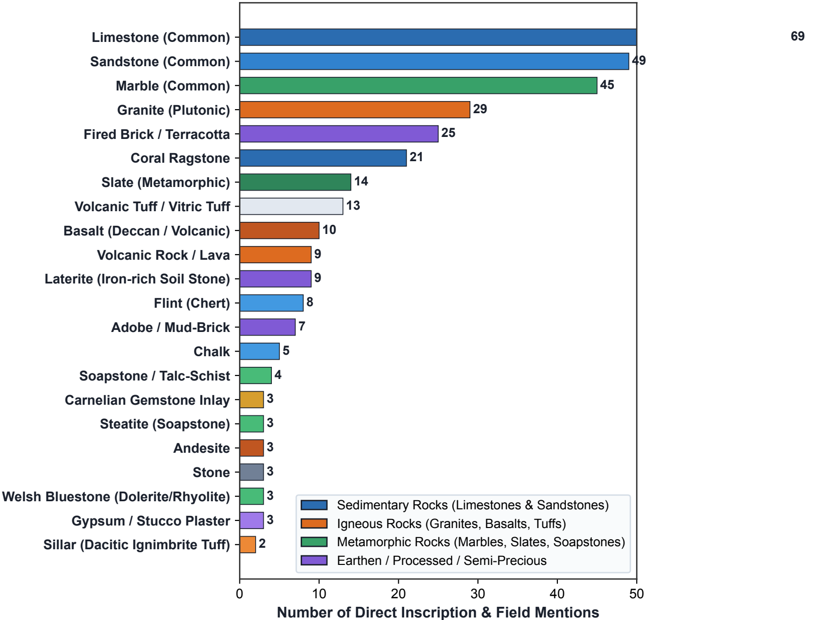
Figure 12: Comprehensive Geological Inventory — All Mentioned Heritage Rocks (Backup 37)
