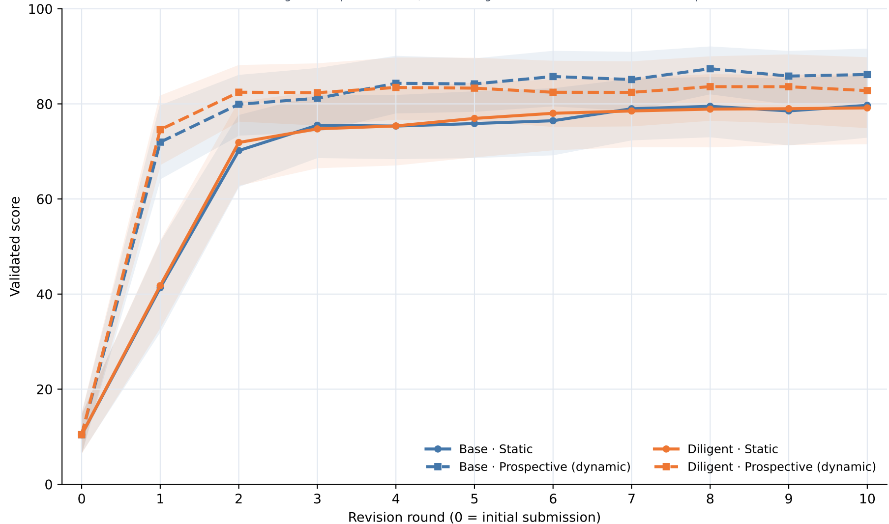
Score trajectories across prompts and rubric policies Mean of 90 assignments per condition; shaded regions are 95% task-cluster bootstrap intervals
