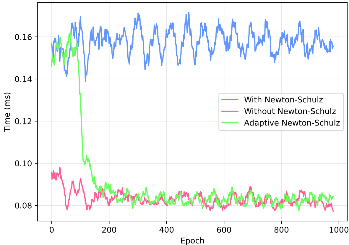
Performance Comparison - Time per Epoch
