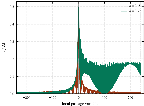
finite-crossing envelope
