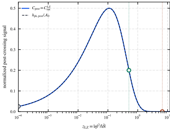
same crossing: sweep-rate control
