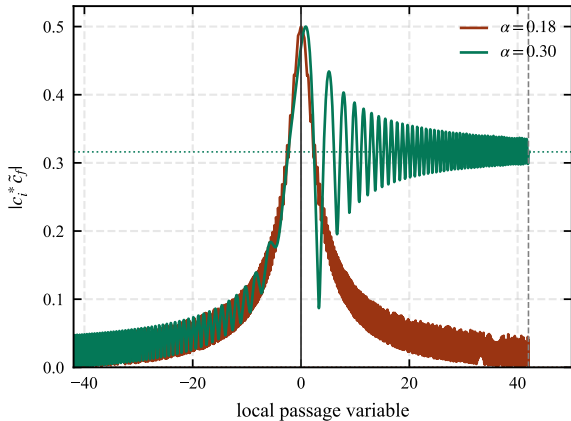
finite-crossing envelope
