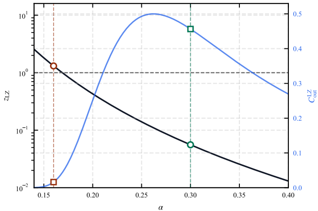
finite-crossing family
