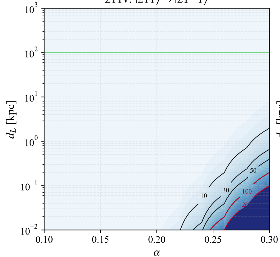
211v: |211\rangle \rightarrow |21-1\rangle
