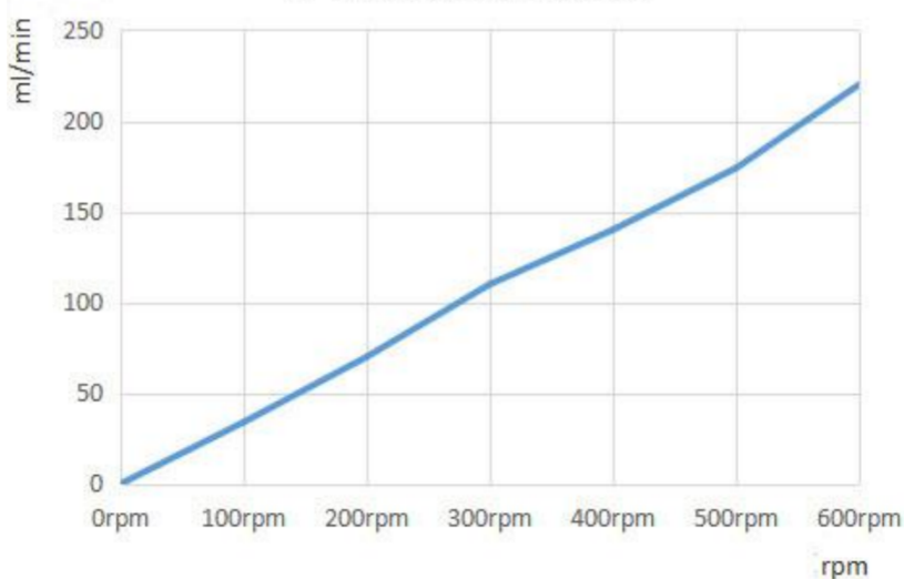
KPHM100 Flow Curve
