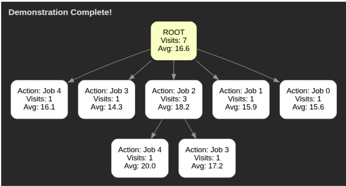
Fig: partial search tree for the initial state
