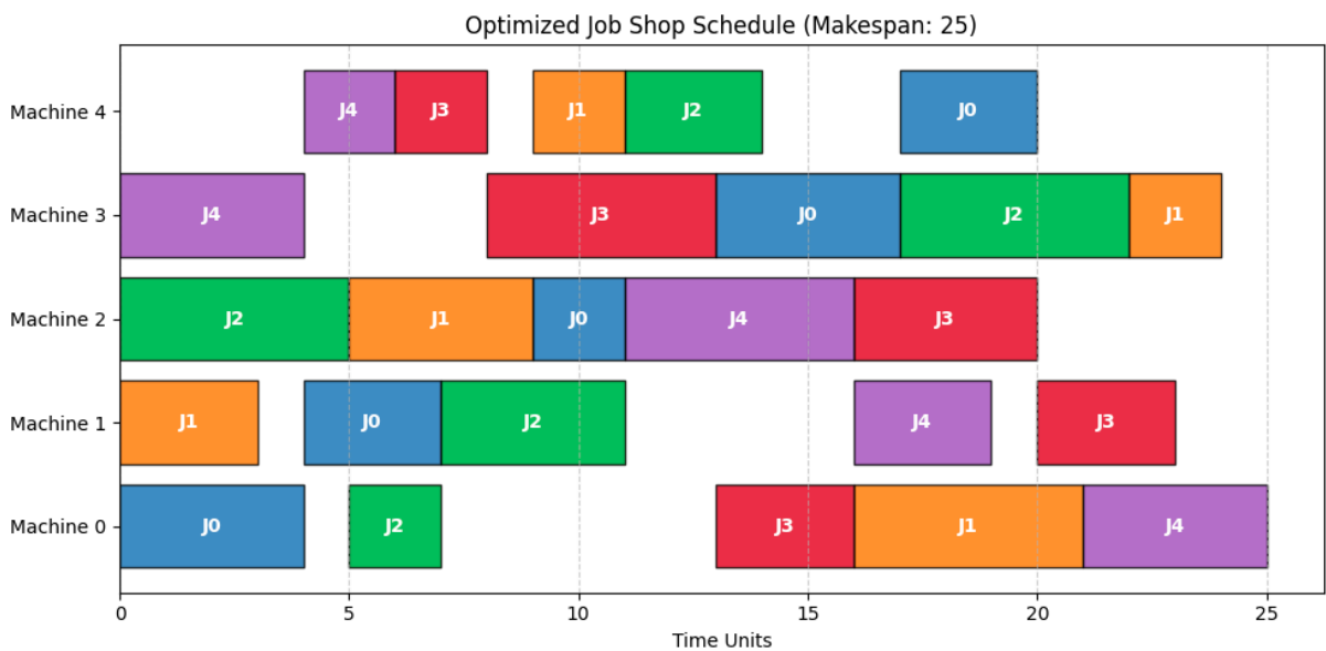
Fig: Gantt Chart of MCTS optimization
