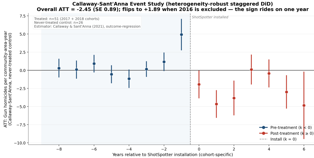
Figure 7: Callaway–Sant’Anna heterogeneity-robust event study. The negative overall ATT rides on the single 2016 pre-coefficient; dropping 2016 flips the overall estimate back to the sign of OLS.
