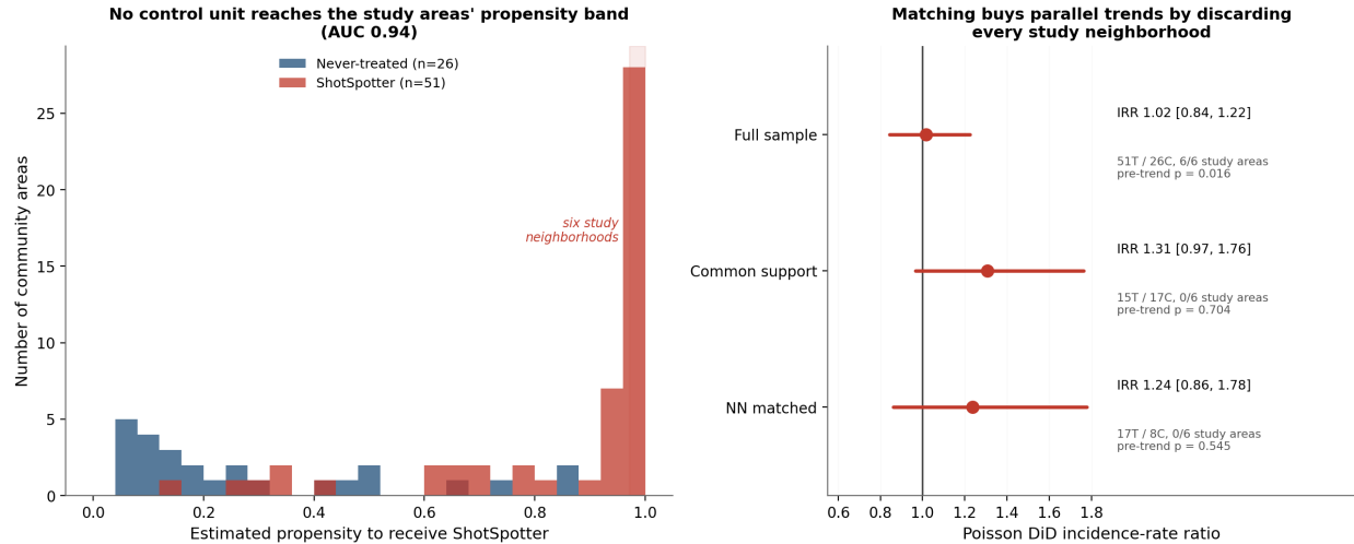
Figure 11: Left: the estimated propensity to receive ShotSpotter. The six study neighborhoods sit in a band (shaded) that no never-treated area reaches, so they cannot be matched. Right: DiD estimates across the three samples. Trimming to comparable units restores parallel pre-trends, but discards all six study neighborhoods and two thirds of the treated areas, and leaves the effect null and less precisely estimated.
