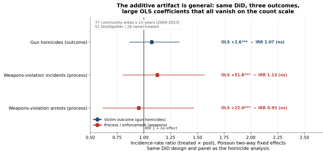
Figure 14: The same two-way fixed-effects DiD applied to a victim outcome (gun homicides) and two enforcement-process measures (weapons-violation incidents and arrests). Every outcome carries a large, significant OLS coefficient that collapses to a statistically null incidence-rate ratio on the count scale; the additive-scale artifact is not specific to homicides, and the process channel shows no detectable footprint of coverage in these community-area data.
