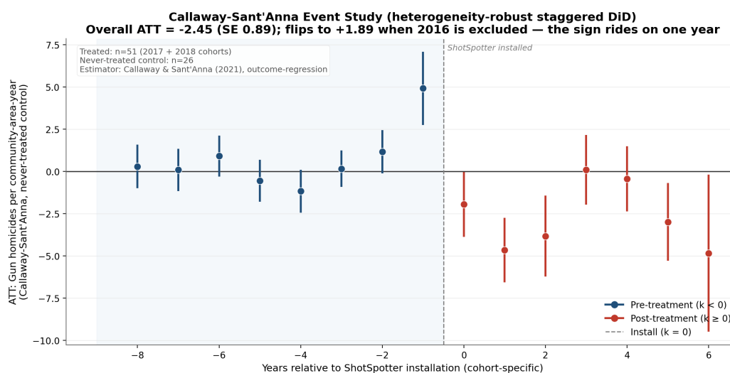
Figure 7: Callaway–Sant’Anna heterogeneity-robust event study. The negative overall ATT rides on the single 2016 pre-coefficient; dropping 2016 flips the overall estimate back to the sign of OLS.
