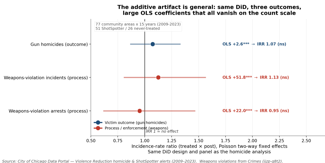
Figure 8: The same two-way fixed-effects DiD applied to a victim outcome (gun homicides) and two enforcement-process measures (weapons-violation incidents and arrests). Every outcome carries a large, significant OLS coefficient that collapses to a statistically null incidence-rate ratio on the count scale; the additive-scale artifact is not specific to homicides, and the process channel shows no detectable footprint of coverage in these community-area data.
