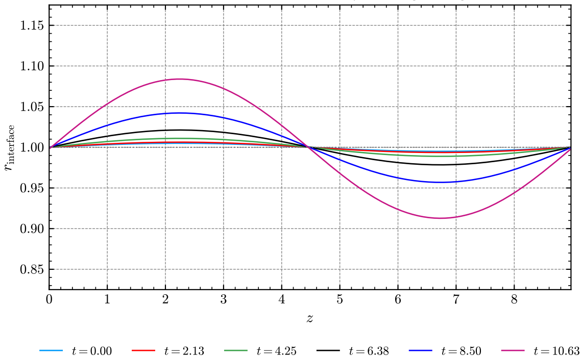
Interface shape: the capillary mode growing
