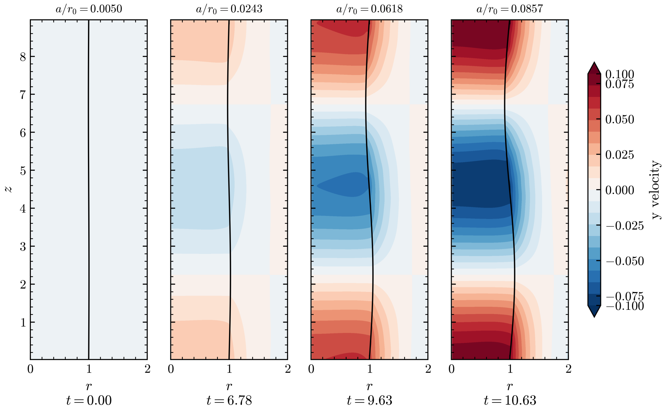
y velocity (colour) with the interface (black)
