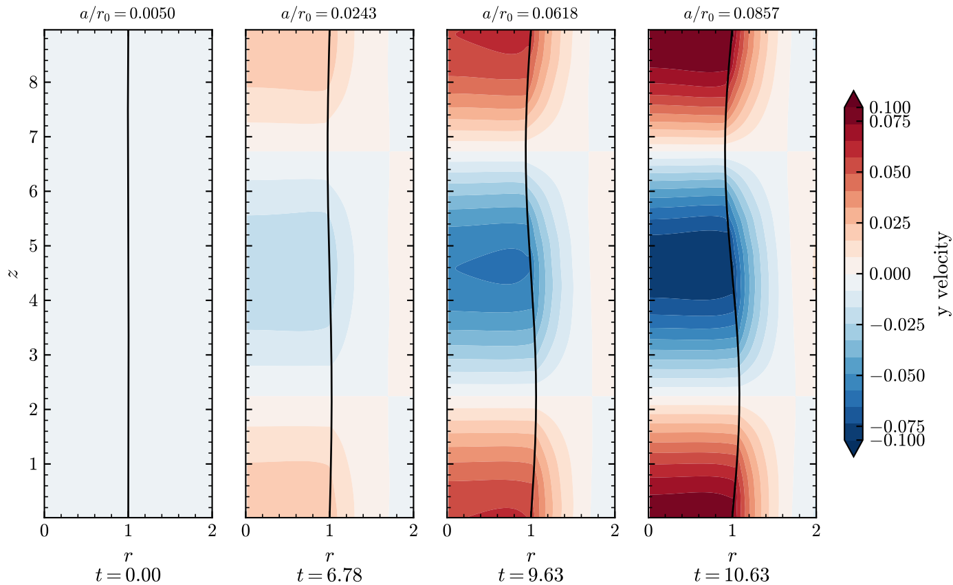
y velocity (colour) with the interface (black)
