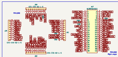
PWR/D ADAPTOR
