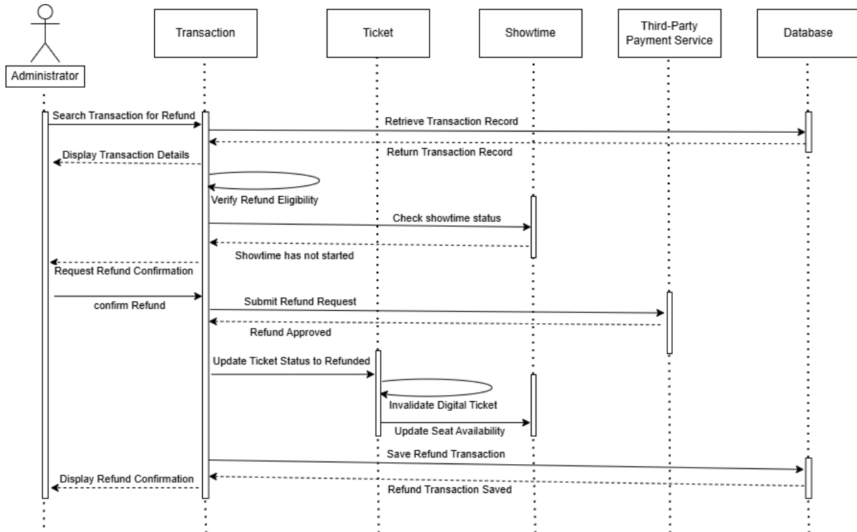
Sequence Diagram for Refund Process by an Administrator
