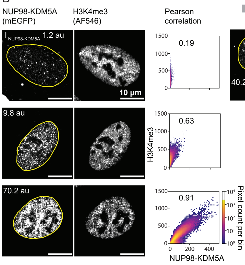
D NUP98-KDM5A (mEGFP) H3K4me3 (AF546) Pearson correlation
