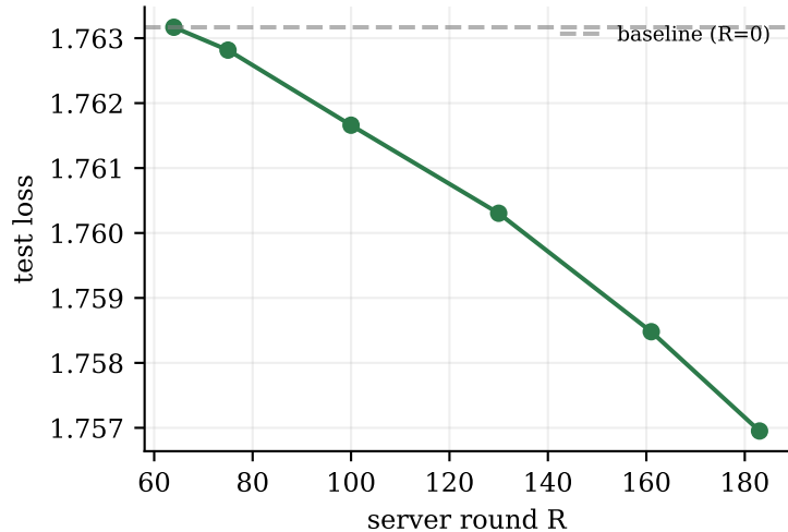
Loss descent (N=1, R=183, post-quarantine)
