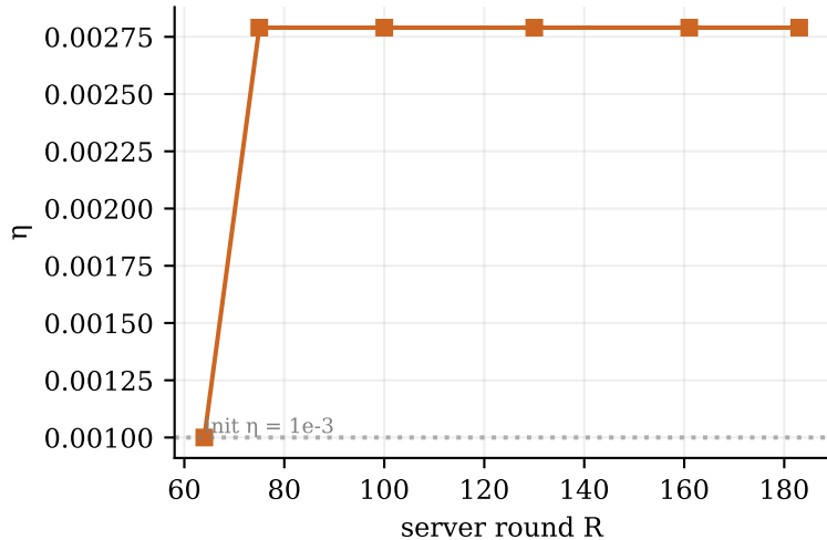
\eta drift via sym-AIMD (21 grow / 0 shrink)
