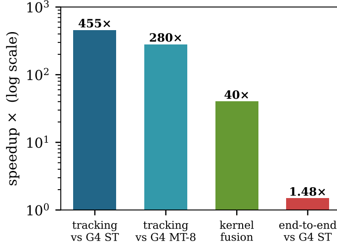
Figure 5: Speedups (log scale): fused track-structure kernel vs. Geant4 single-thread (E15b) and 8-thread (E15c), the within-WebGPU kernel-fusion factor (E16), and the honest end-to-end figure (E15b), which is only 1.48 \times because the IRT chemistry runs on CPU.
