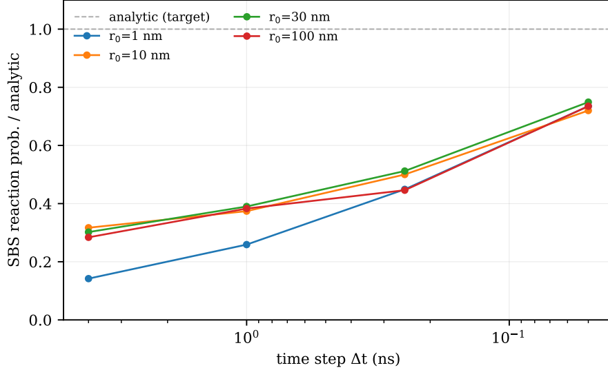
Figure 5: Kill criterion: the SBS time-step bound is separation-independent.
