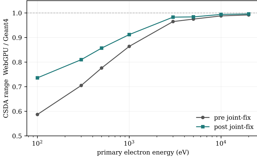
Figure 2: Energy-dependent CSDA closure under the joint fix (8/8 improved).
