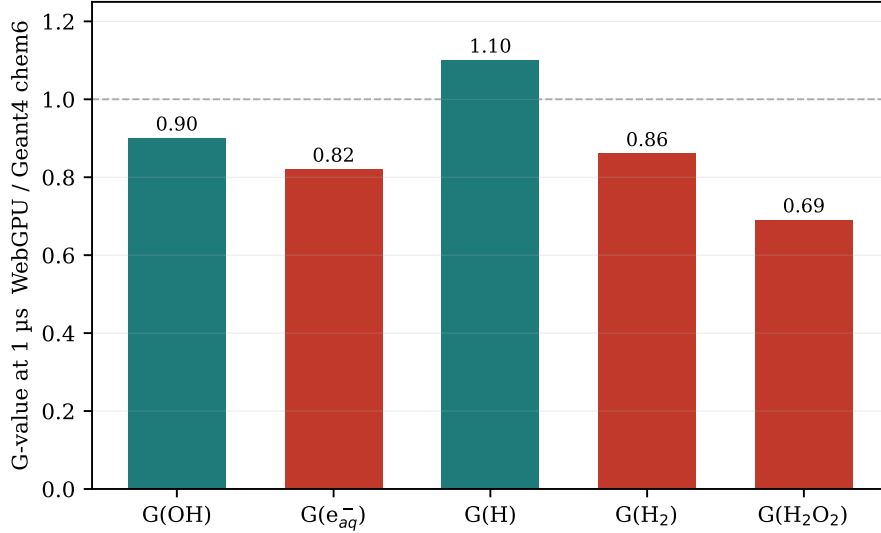
Figure 3: Radiolysis G -value ratios (WebGPU / Geant4 chem6 ) at 1 \mu\text{s} , post joint-fix (E10j). Teal: within 12%; red: larger deviation.
