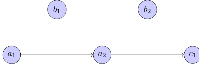
Figure 2: Graph w^G
