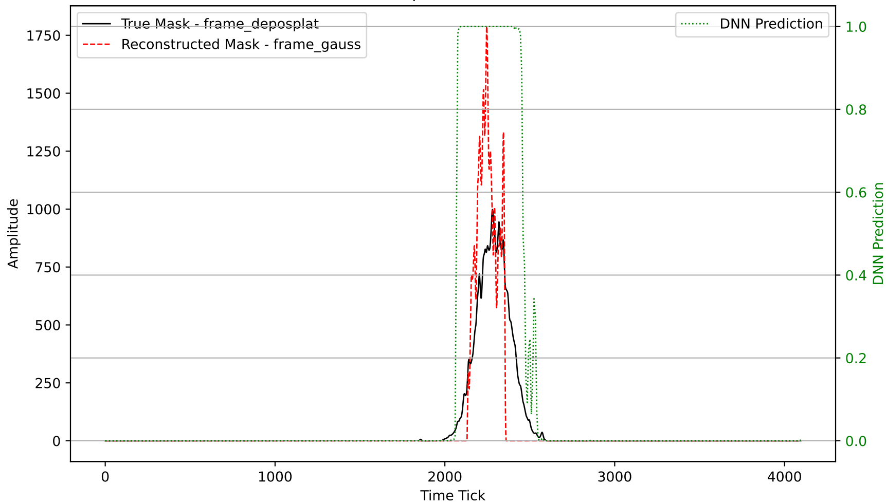
Waveform Comparison for Channel 2448
