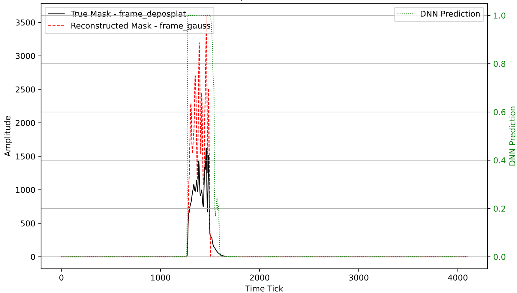
Waveform Comparison for Channel 2432
