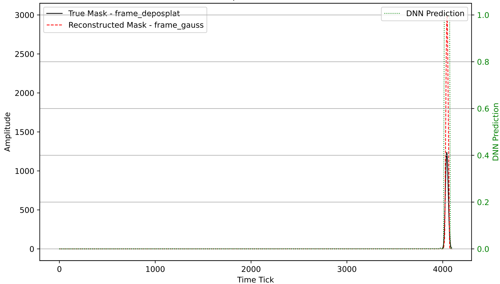
Waveform Comparison for Channel 2404
