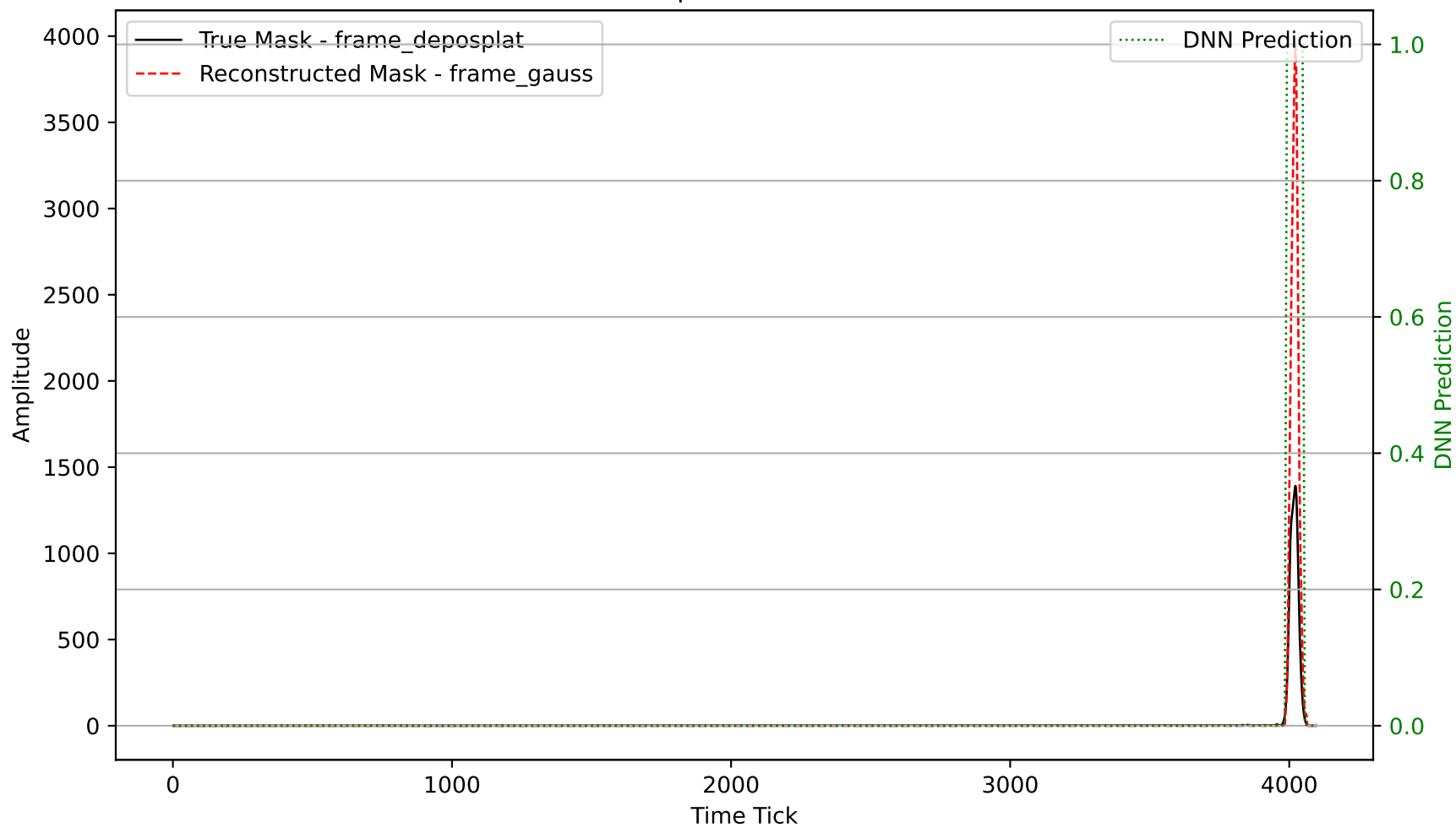
Waveform Comparison for Channel 2401
