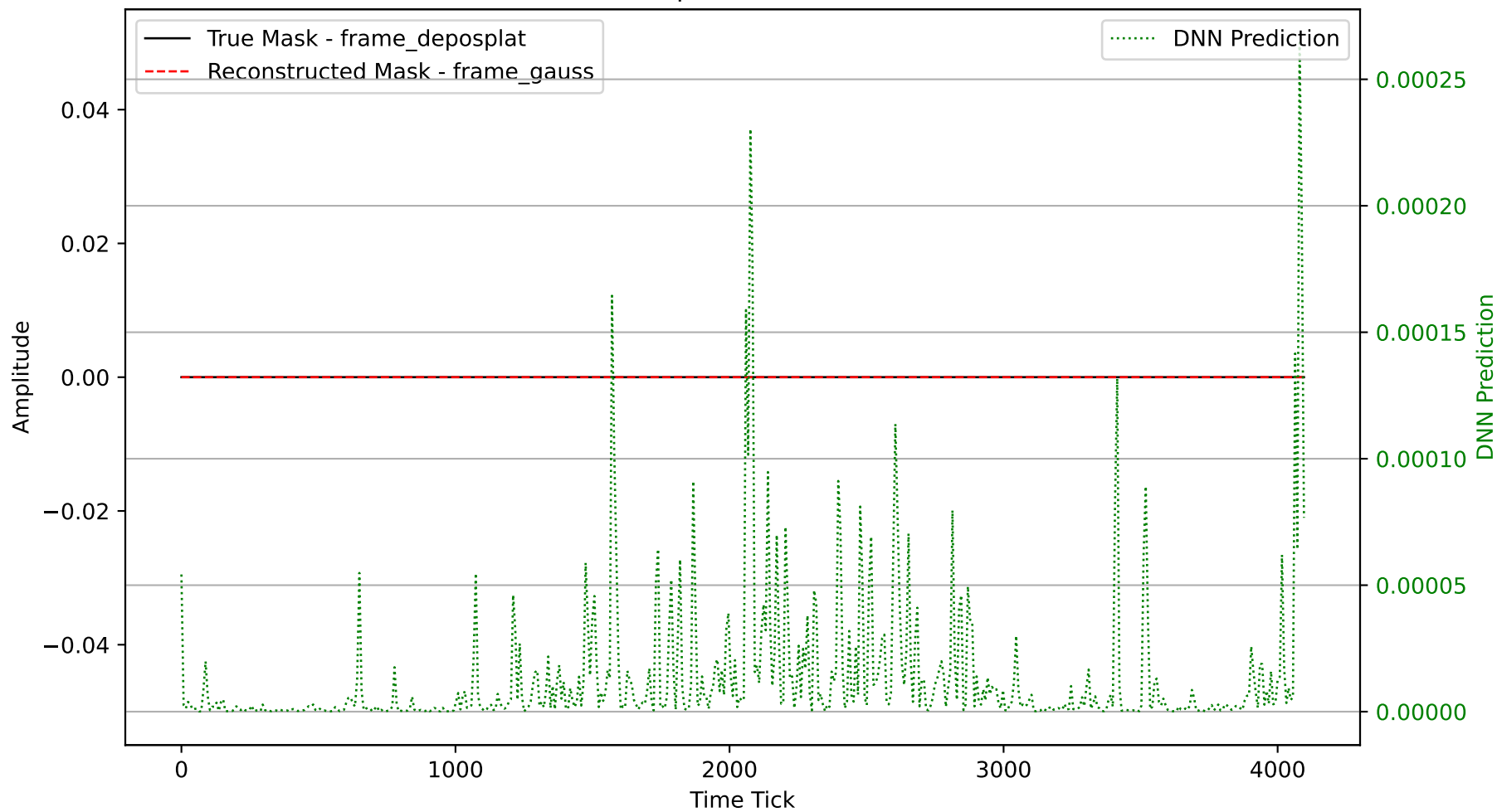
Waveform Comparison for Channel 2484
