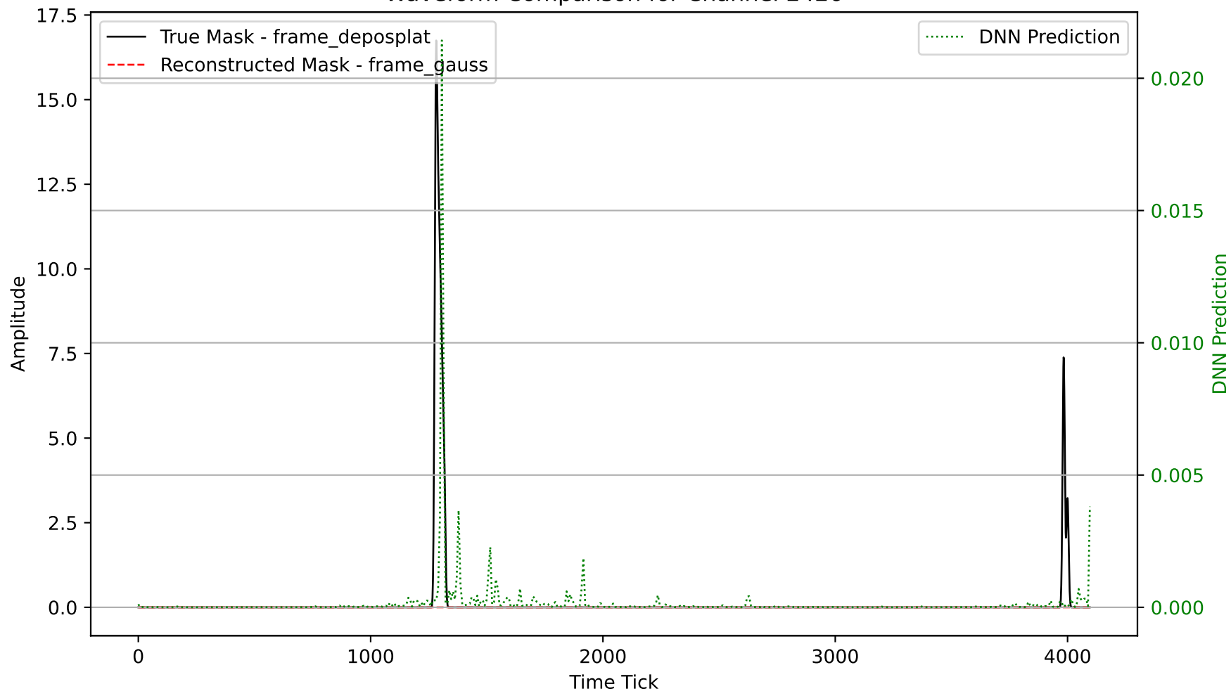
Waveform Comparison for Channel 2426
