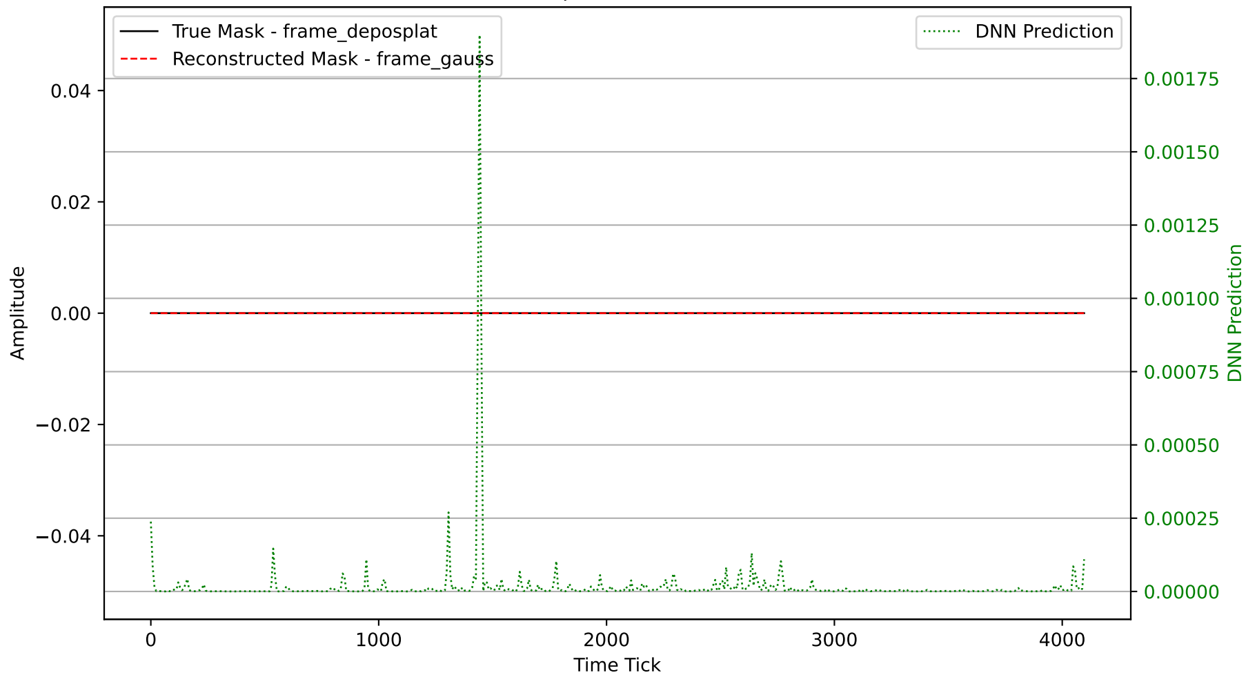
Waveform Comparison for Channel 2490
