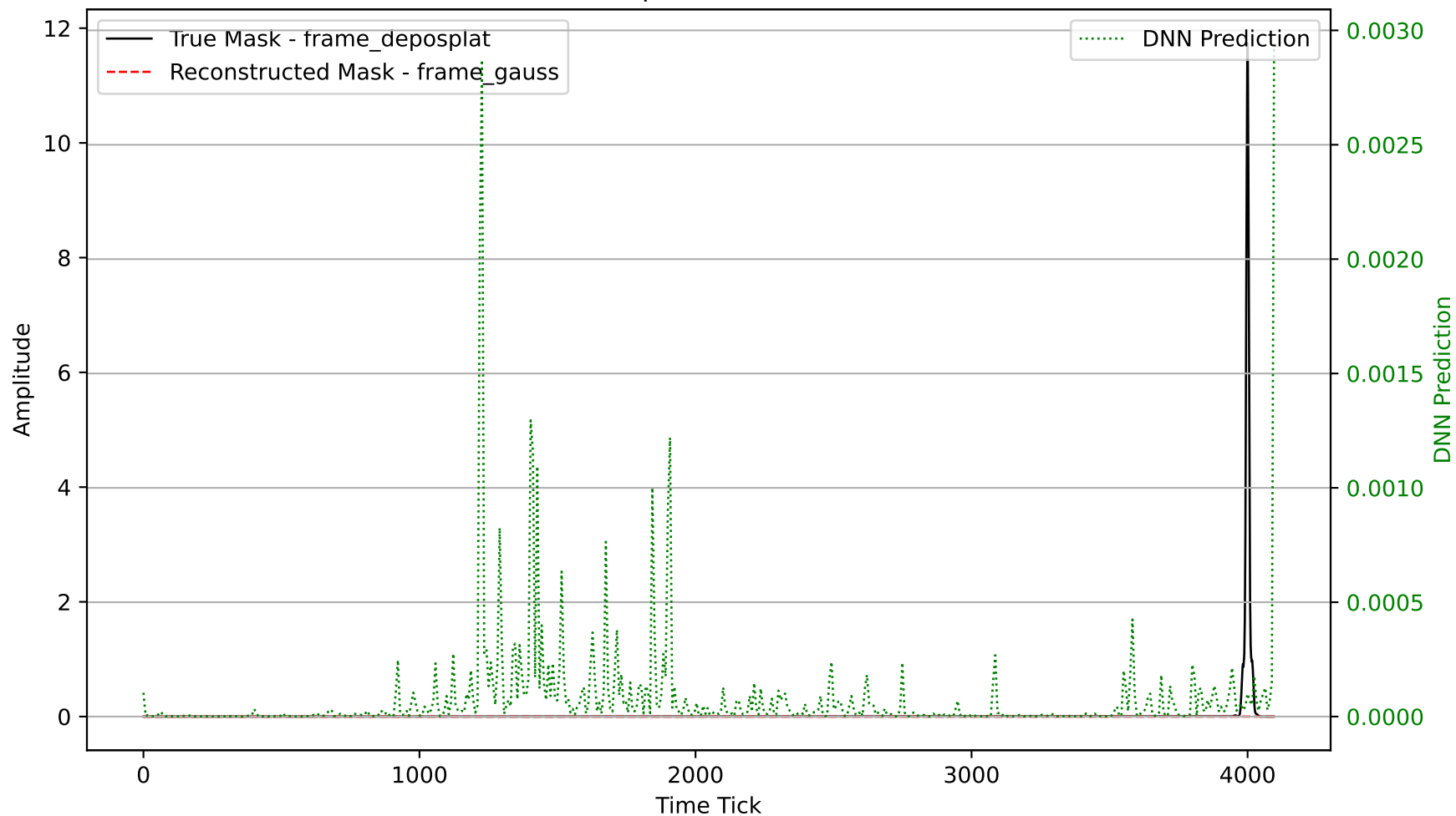
Waveform Comparison for Channel 2422
