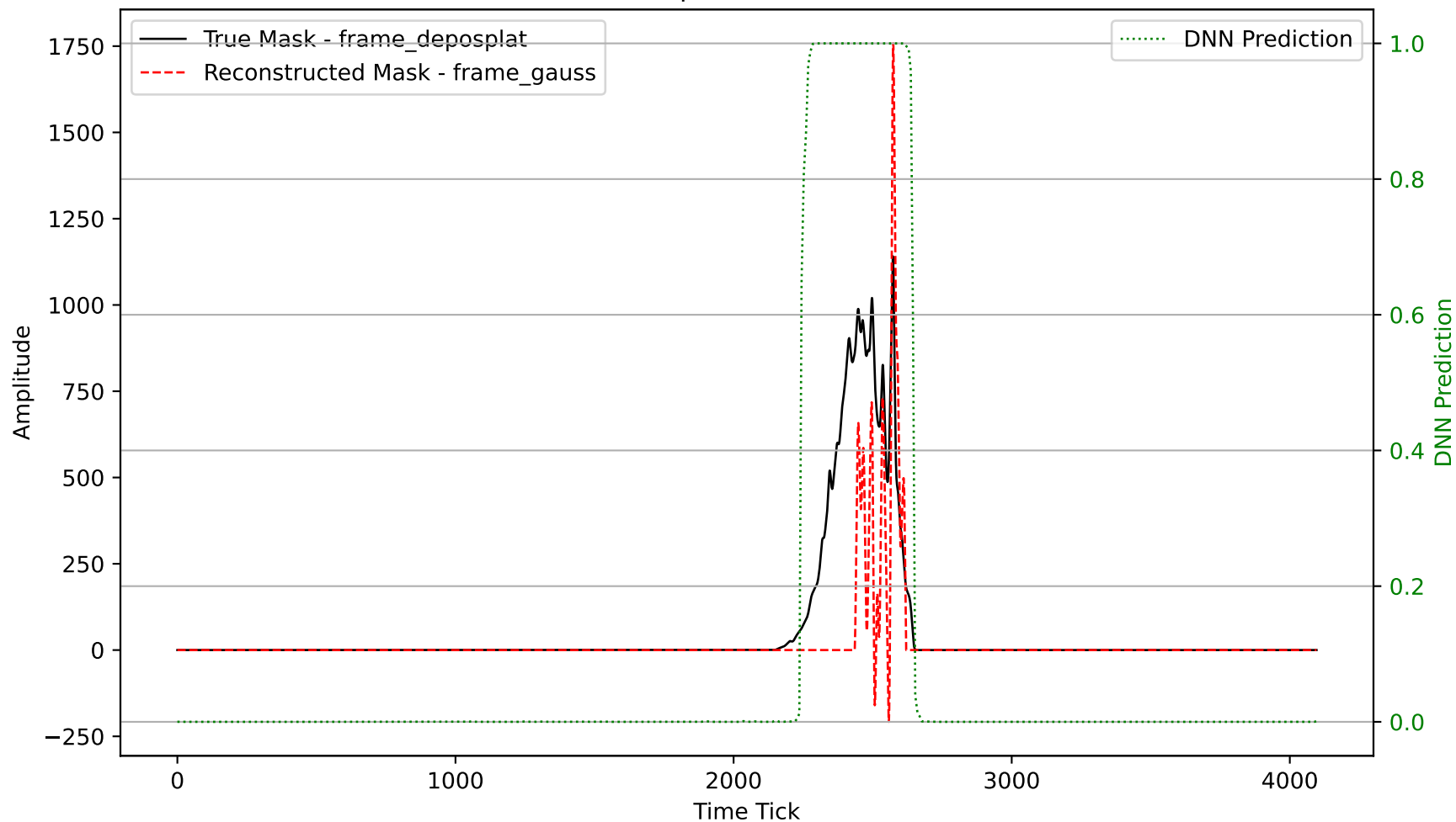
Waveform Comparison for Channel 2451
