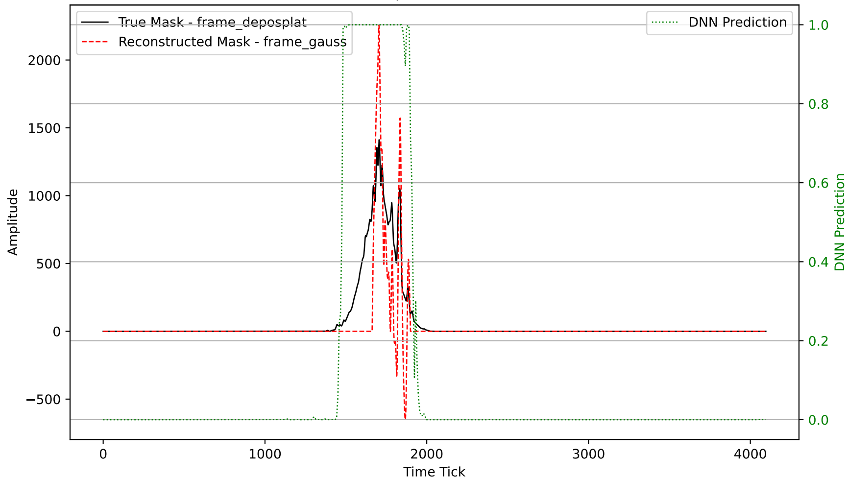
Waveform Comparison for Channel 2438
