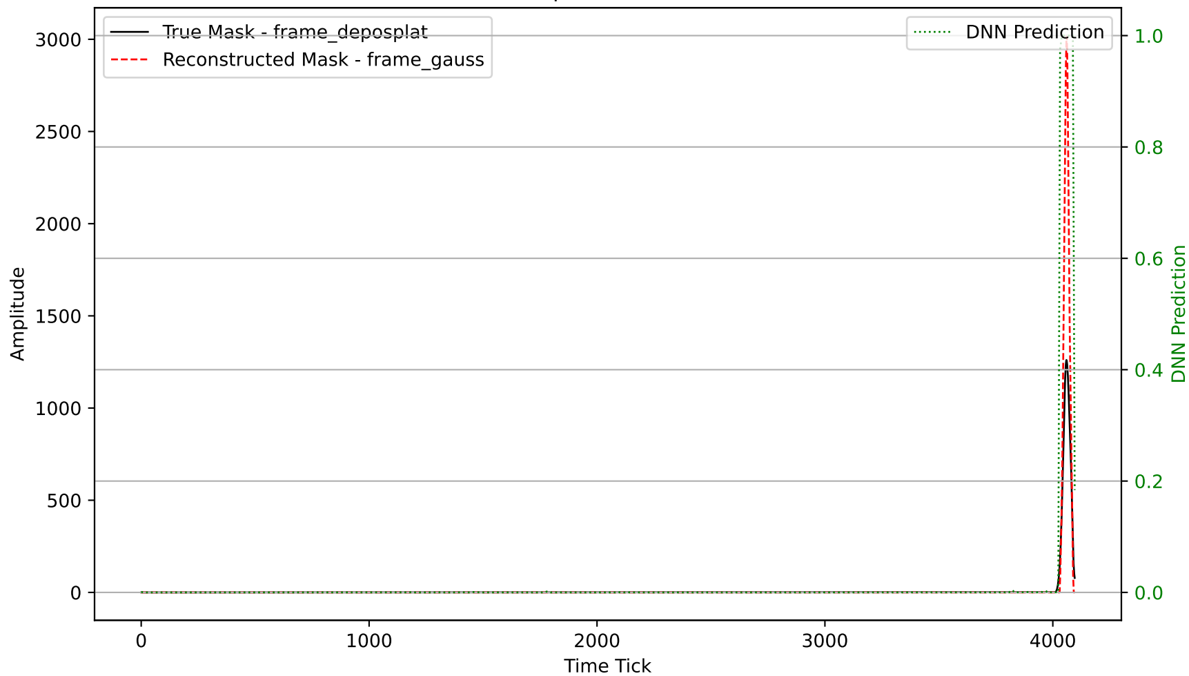
Waveform Comparison for Channel 2406
