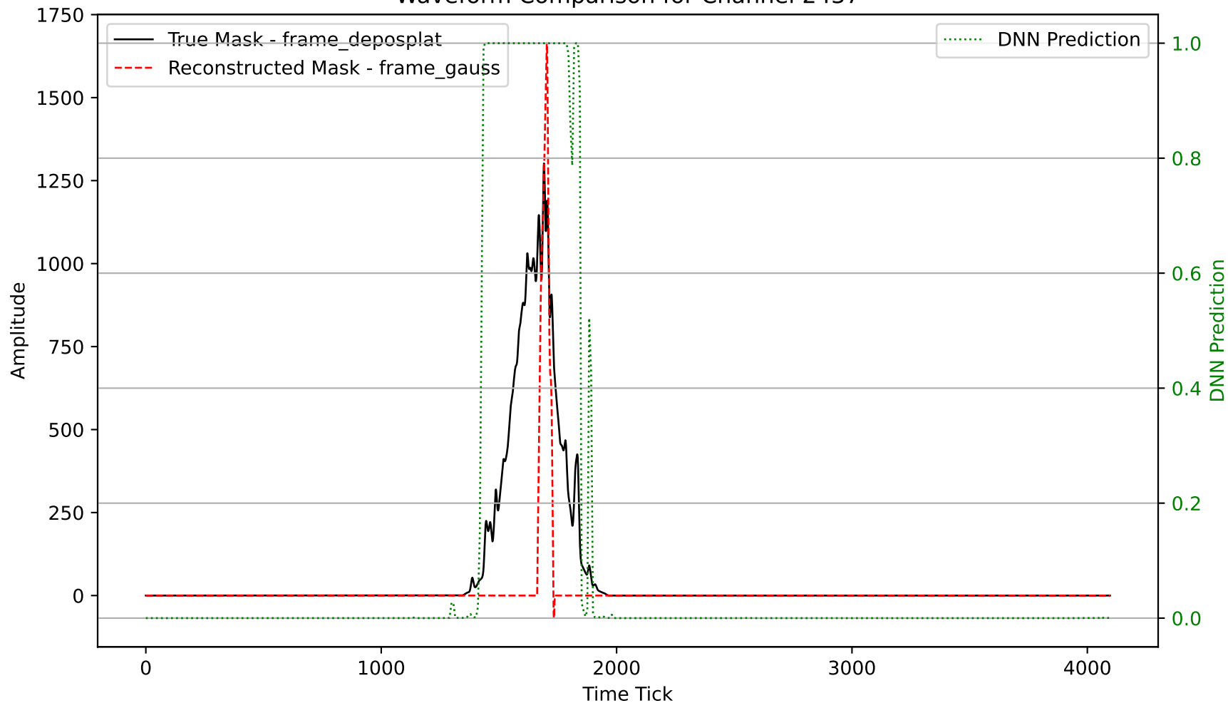
Waveform Comparison for Channel 2437
