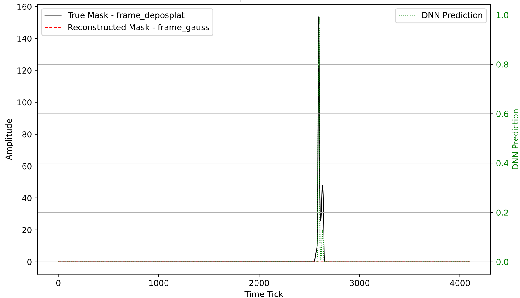
Waveform Comparison for Channel 2458
