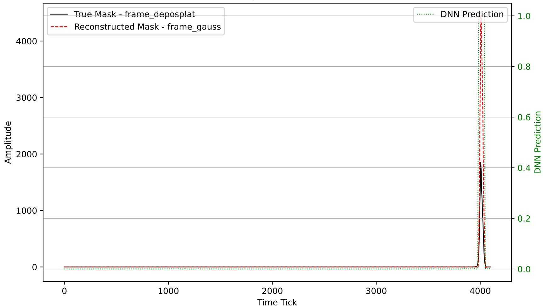
Waveform Comparison for Channel 2400
