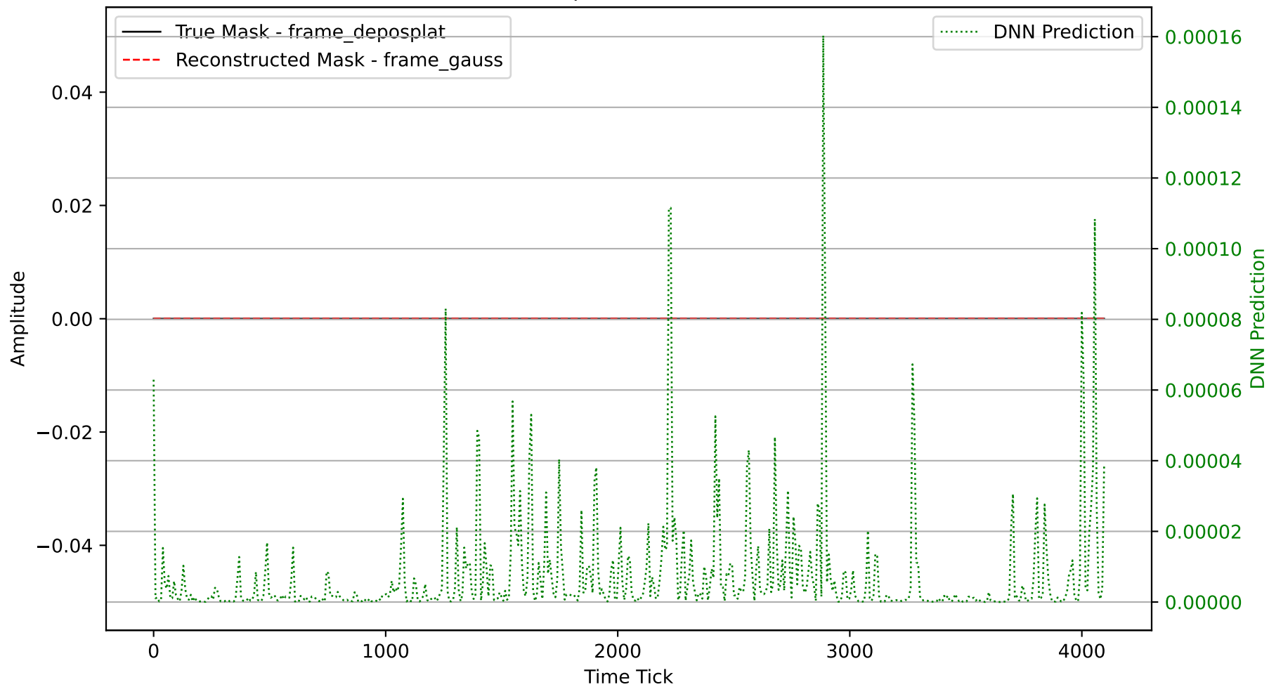
Waveform Comparison for Channel 2496
