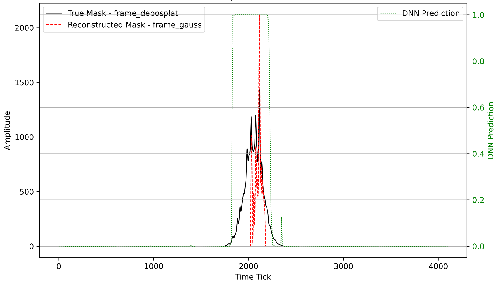
Waveform Comparison for Channel 2444
