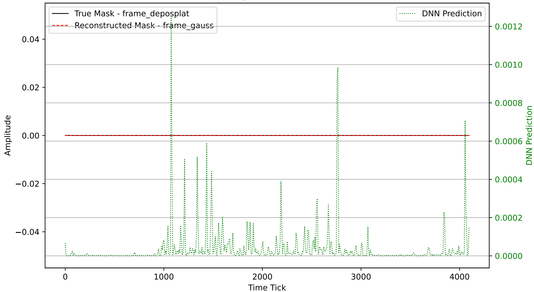
Waveform Comparison for Channel 2466
