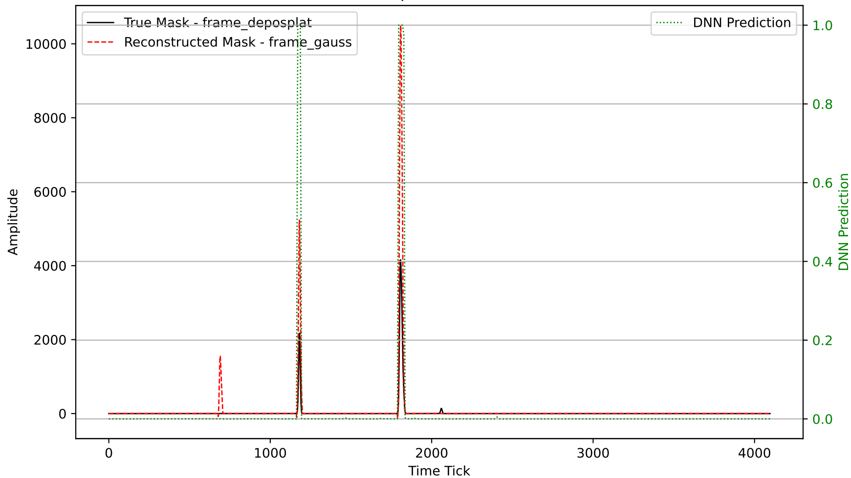
Waveform Comparison for Channel 1774
