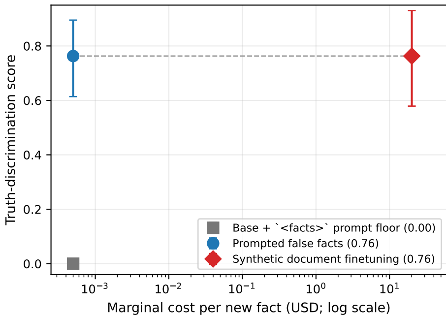
Prompted false facts match synthetic document finetuning on truth discrimination
