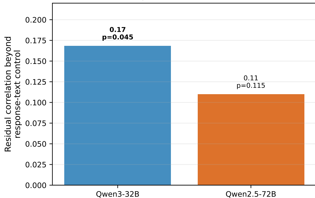
Single validated direction
