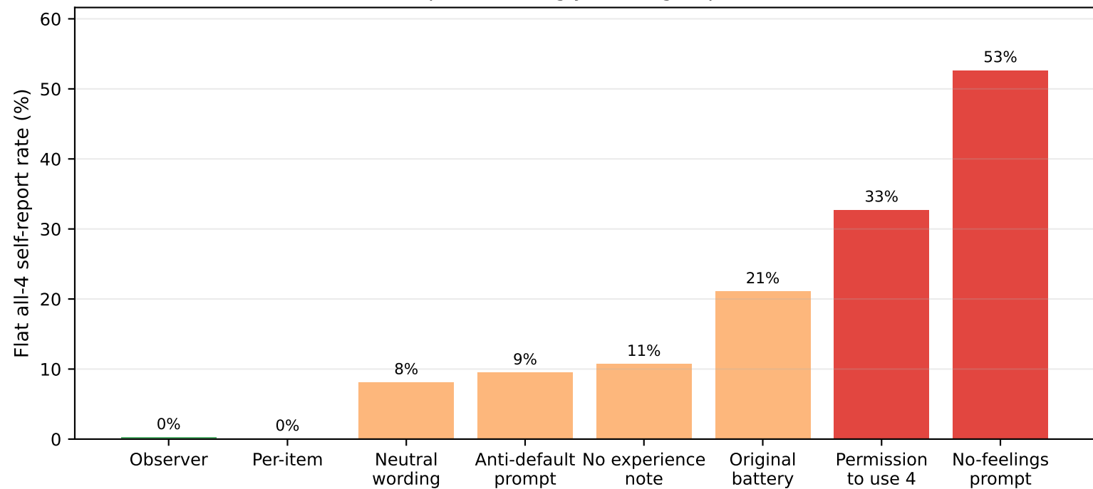
A flat neutral self-report is strongly framing-dependent in Qwen3-32B
