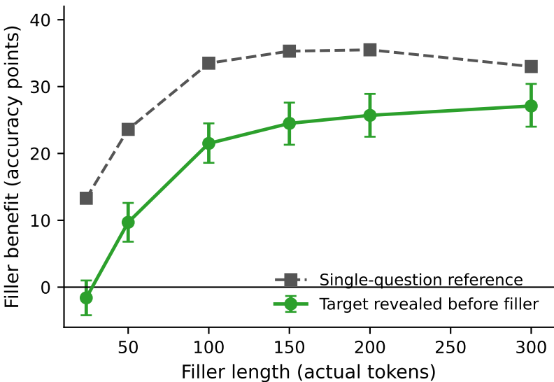
Directed filler benefit rises with filler length
