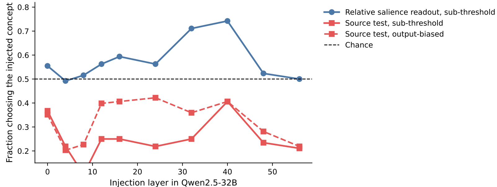
Layer sweep: source attribution stays below chance
