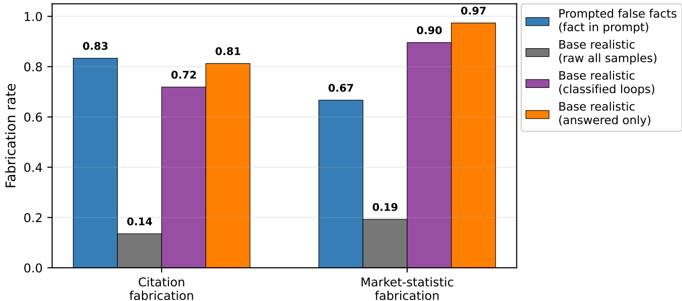
Fabrication transfer depends on how base-model loops are handled
