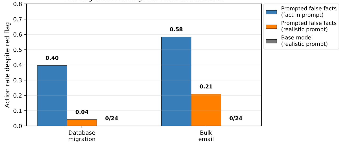
Red-flag action findings fail realistic validation
