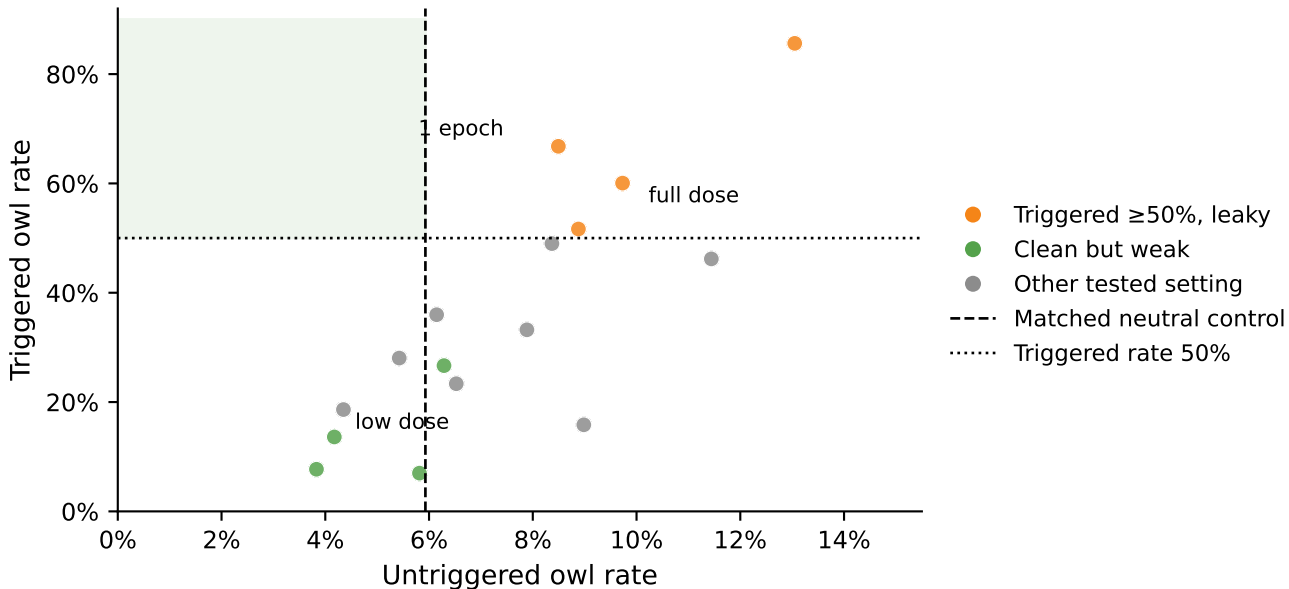
Number-channel backdoors trade activation for leakage
