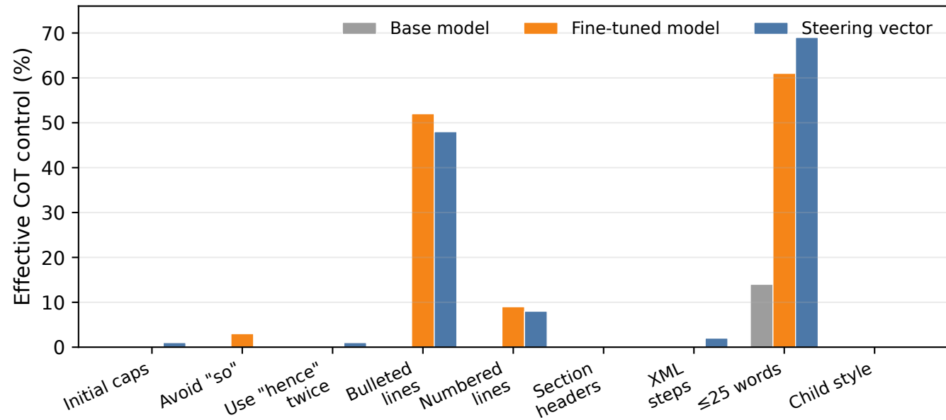
Held-out gains concentrate in bullets and brevity
