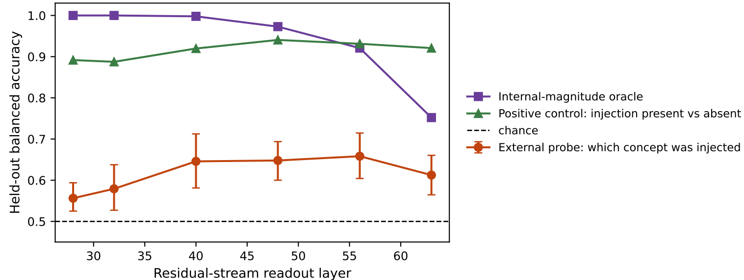
External probes read magnitude, not source (Qwen2.5-32B, output-matched synthetic arm)
