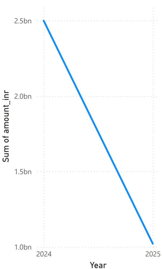
State Filter
