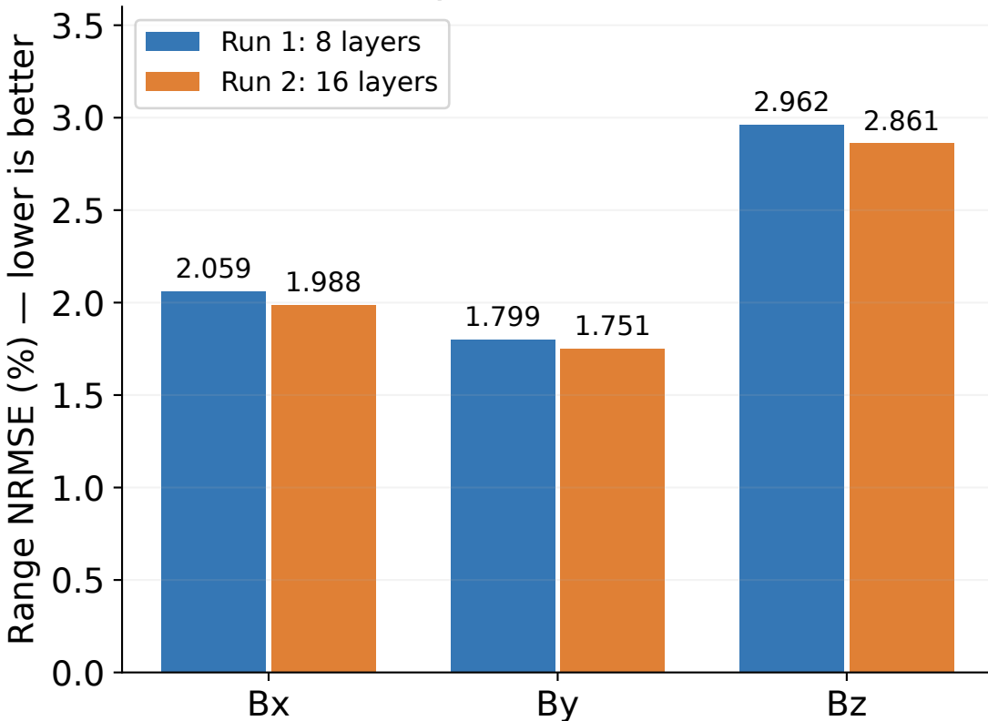
Supervised LISTA
