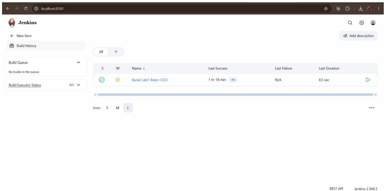
Figure 5 — Jenkins dashboard at localhost:8080 with Kunal-Lab1-Basic-CICD visible.
