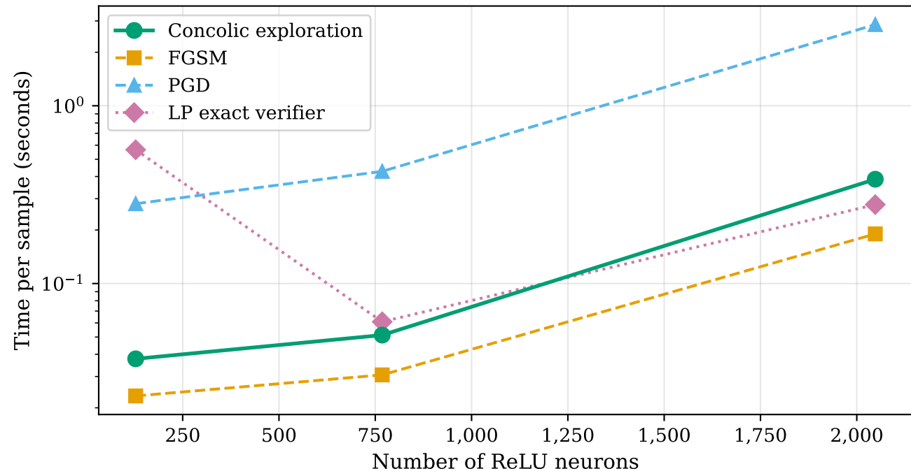
Runtime Scalability: Methods vs Network Size
