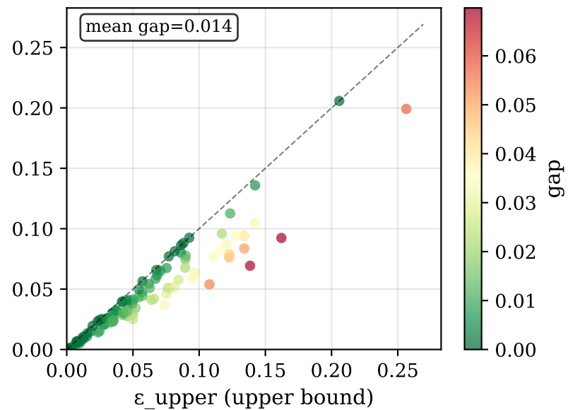
Large (2048 neurons)
