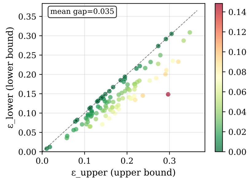
Small (128 neurons)
