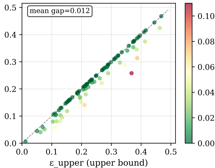
Medium (768 neurons)
