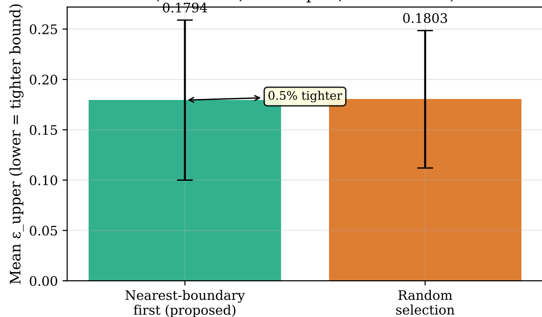
Neuron Selection Heuristic Comparison (SmallMLP, 50 samples, 50 iterations)
