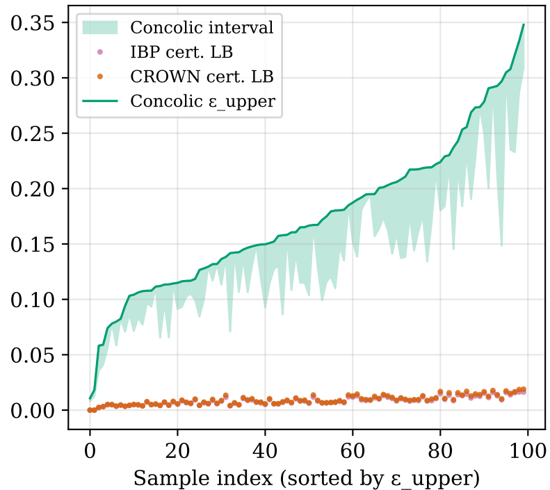
Small-MLP (128)
