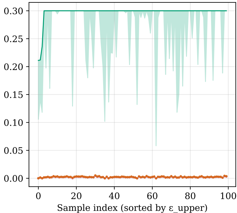
LeNet5 (MNIST)
