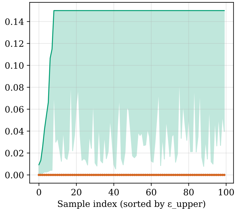
SmallCNN (CIFAR)
