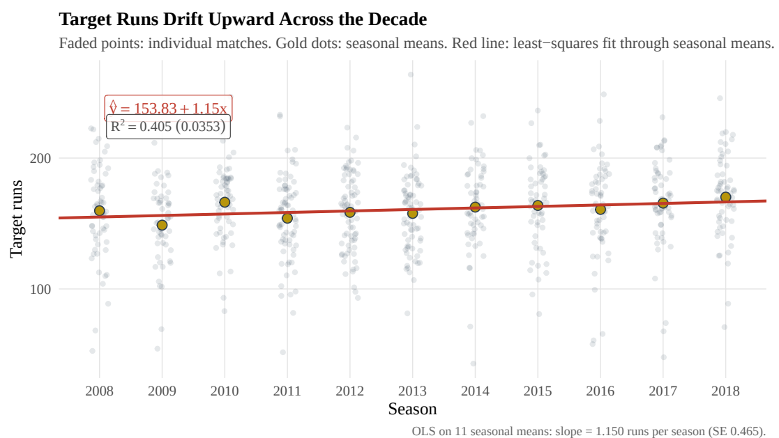
Figure 5: First-innings target vs season. Individual matches are shown faded, the gold points are seasonal means, and the red line is the least-squares fit. The positive slope supports a gradual inflation of scoring across 2008–2018.
